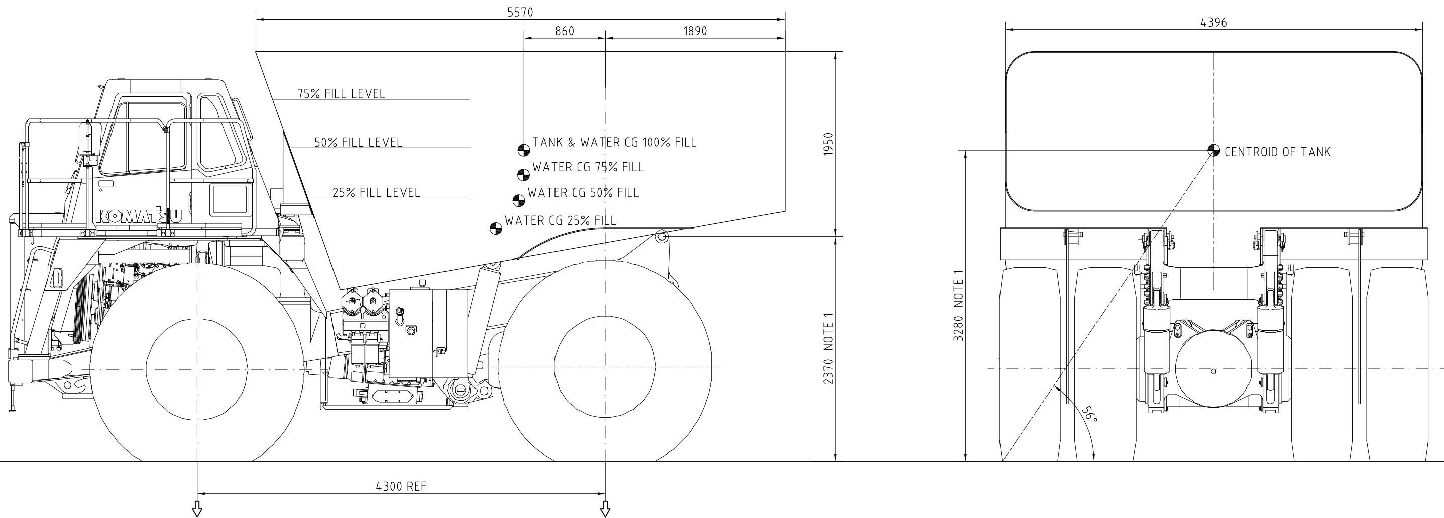
KOMATSU HD465-7 TRUCK W/ KADOR 45kl WATER TANK
