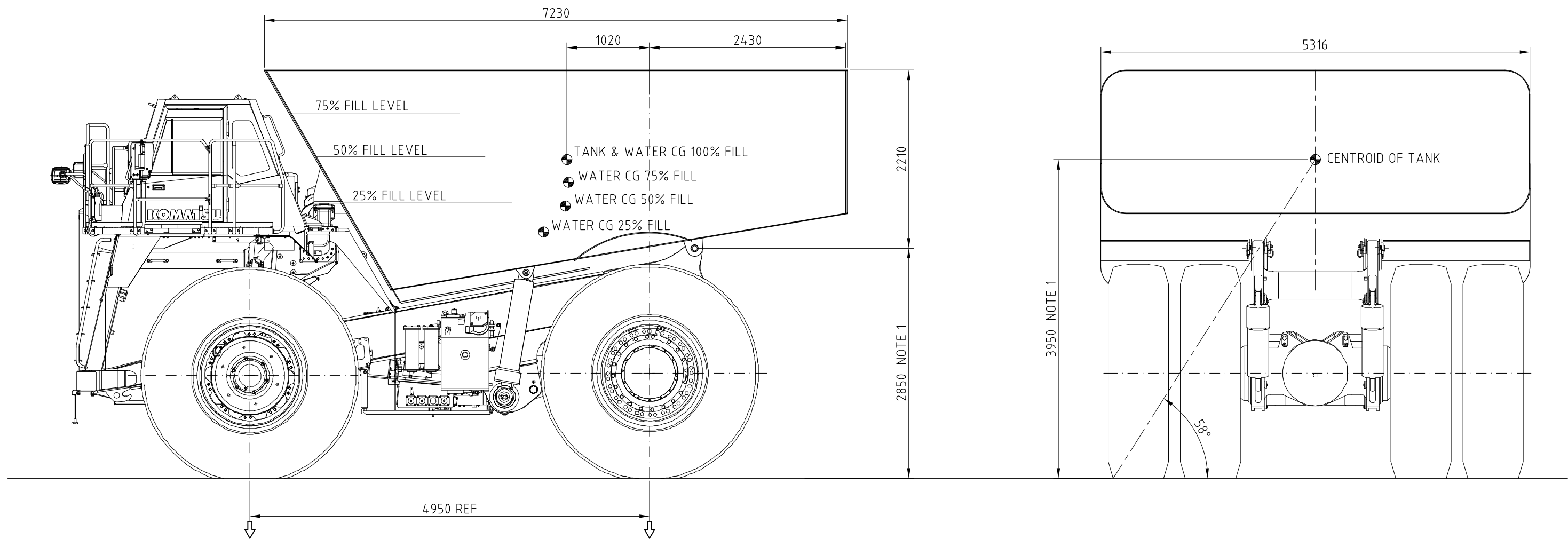
KOMATSU HD785-7 TRUCK W/ KADOR 75kl WATER TANK
